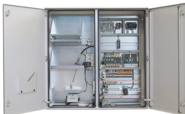
Stainless steel cabinets with electrical equipment, made in accordance with the design provided by the client
